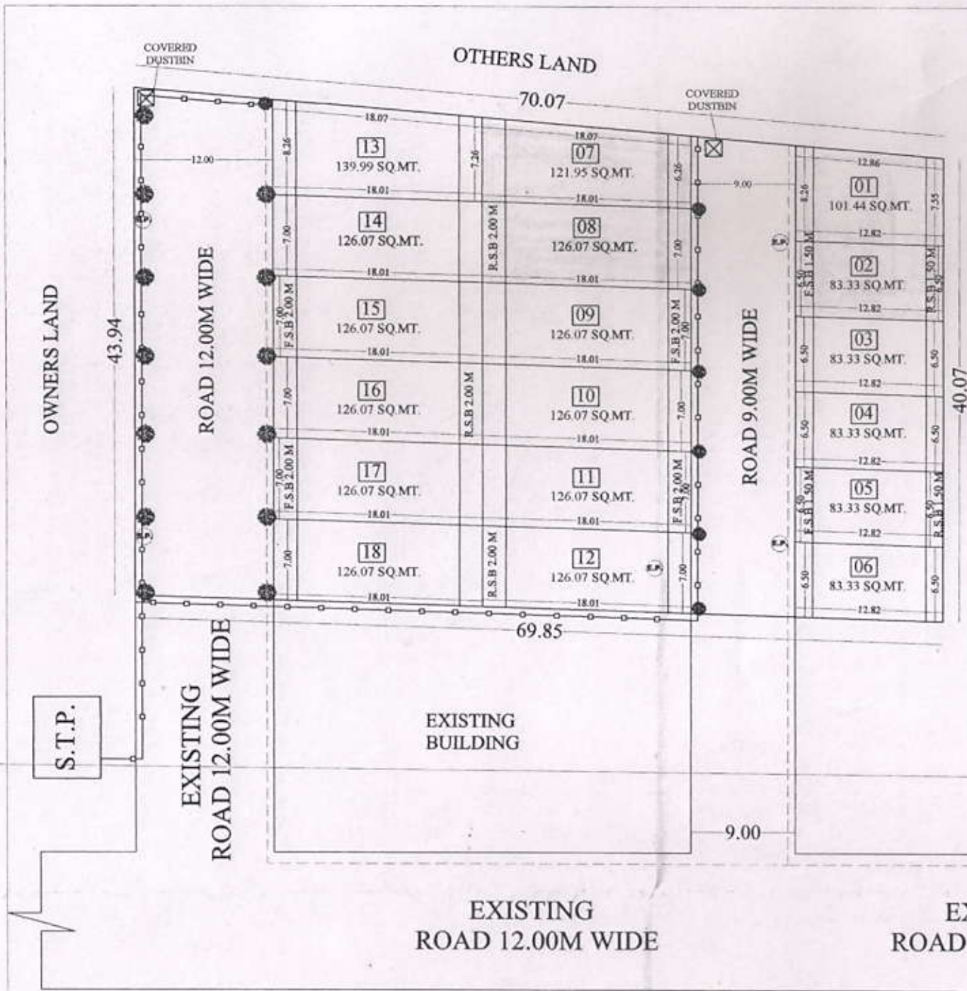
SITE LAYOUT PLAN SCALE 1:200
